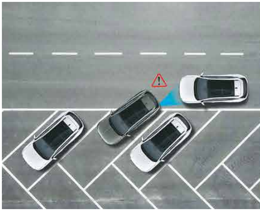
Rear cross traffic collision avoidance assist (RCCA)
